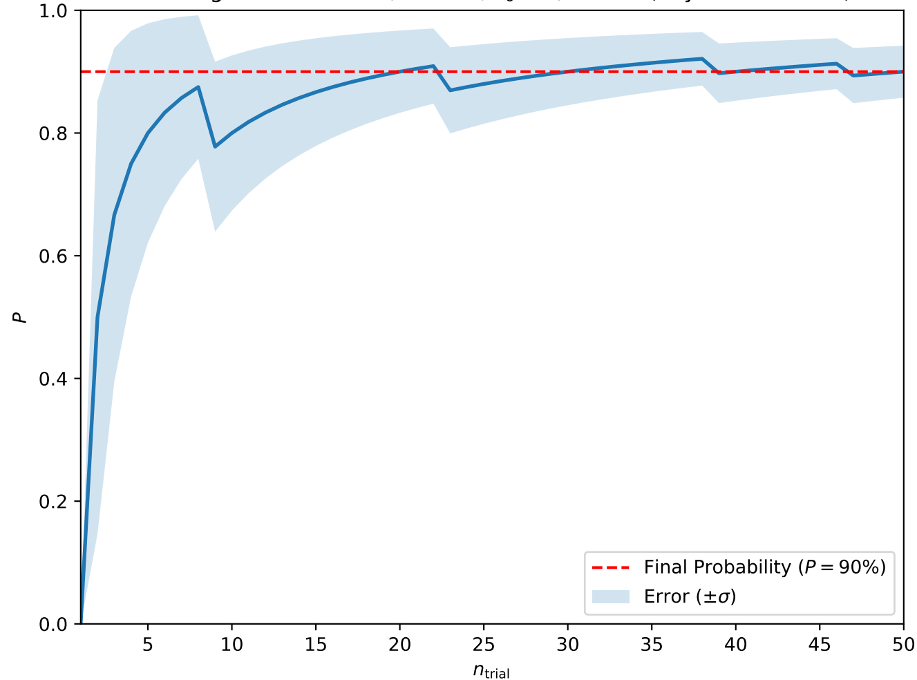
Convergence at A = 0.2, H = 0.4, T_0 = 3, w = 10 (Skyrmion Lattice)
