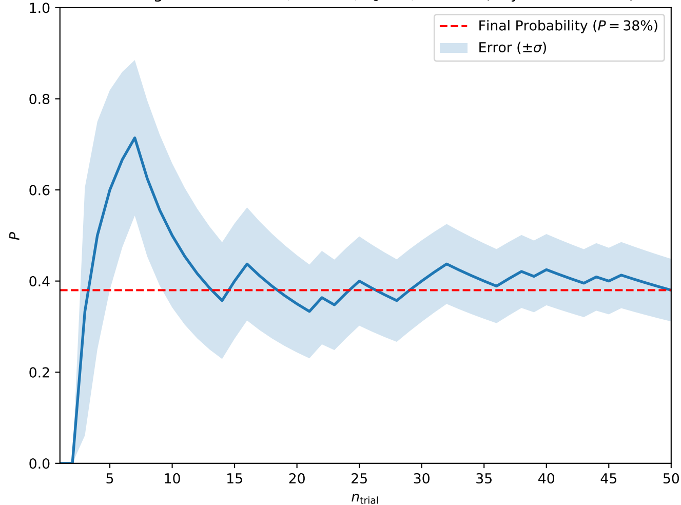
Convergence at A = 0.2, H = 0.4, T_0 = 3, w = 2.5 (Skyrmion Lattice)
