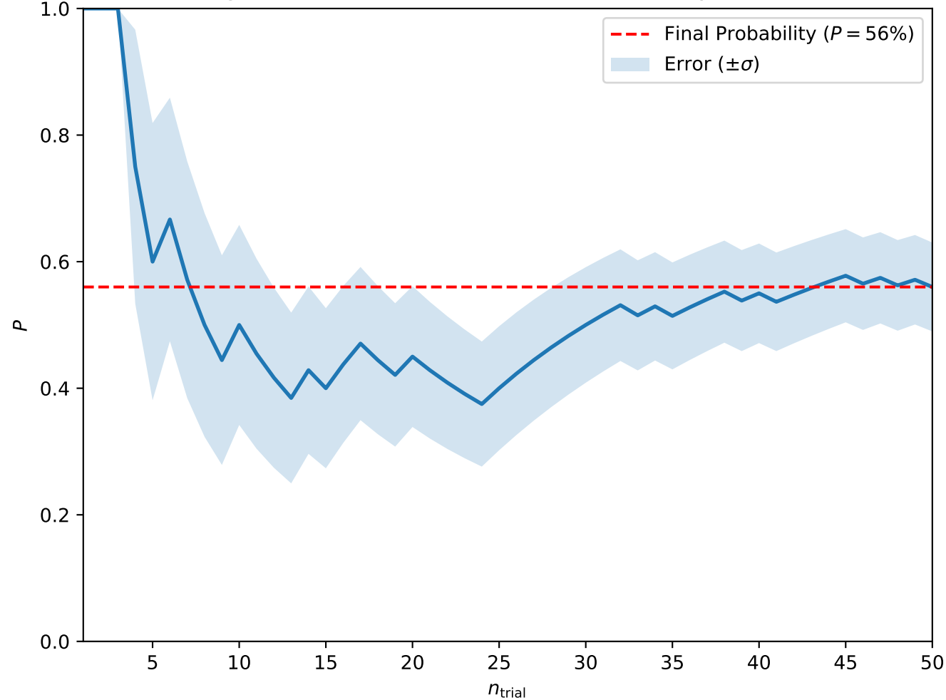
Convergence at A = 0.2, H = 0.4, T_0 = 3, w = 5 (Skyrmion Lattice)
