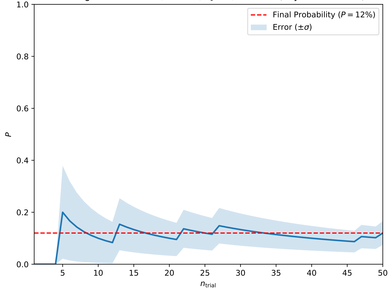
Convergence at A = 0.2, H = 0.4, T_0 = 5, w = 1.25 (Skyrmion Lattice)
