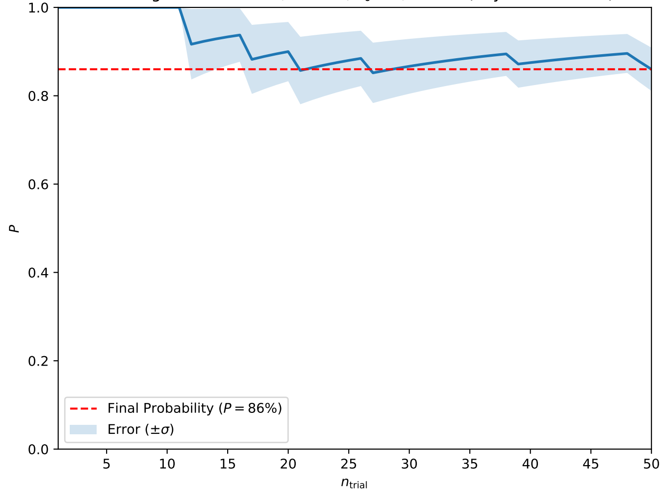
Convergence at A = 0.2, H = 0.4, T_0 = 5, w = 10 (Skyrmion Lattice)
