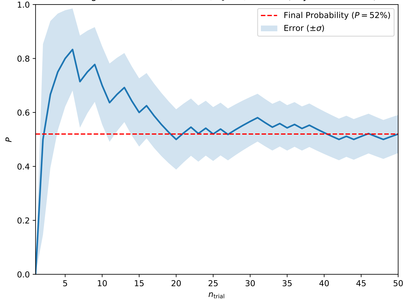
Convergence at A = 0.2, H = 0.4, T_0 = 5, w = 2.5 (Skyrmion Lattice)
