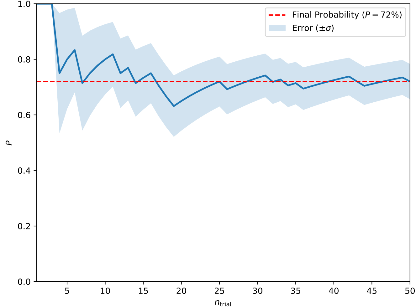
Convergence at A = 0.2, H = 0.4, T_0 = 5, w = 5 (Skyrmion Lattice)
