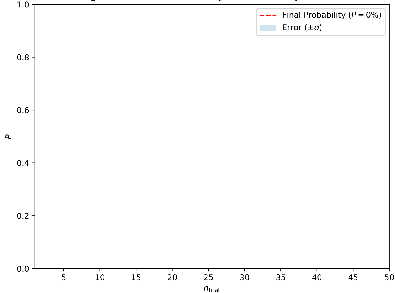
Convergence at A = 0.2, H = 0.5, T_0 = 1, w = 10 (Skyrmion Lattice)
