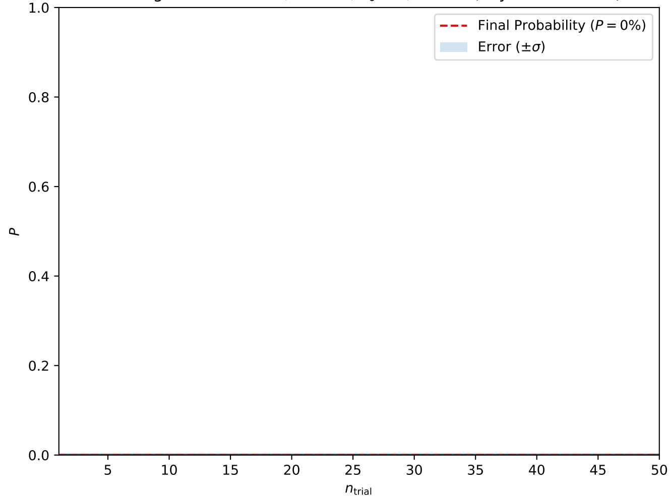
Convergence at A = 0.2, H = 0.5, T_0 = 3, w = 10 (Skyrmion Lattice)
