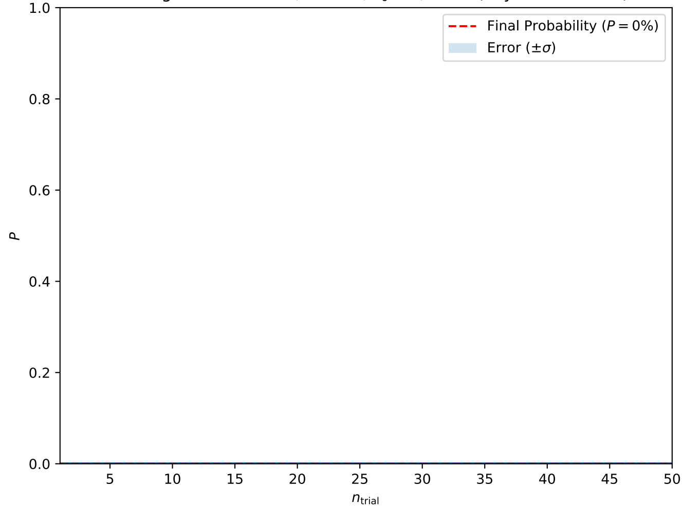
Convergence at A = 0.2, H = 0.5, T_0 = 3, w = 5 (Skyrmion Lattice)
