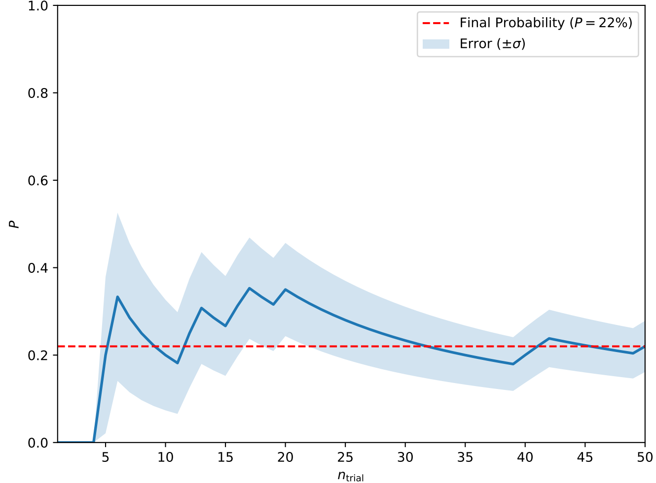
Convergence at A = 0.3, H = 0.3, T_0 = 1, w = 10 (Skyrmion Lattice)
