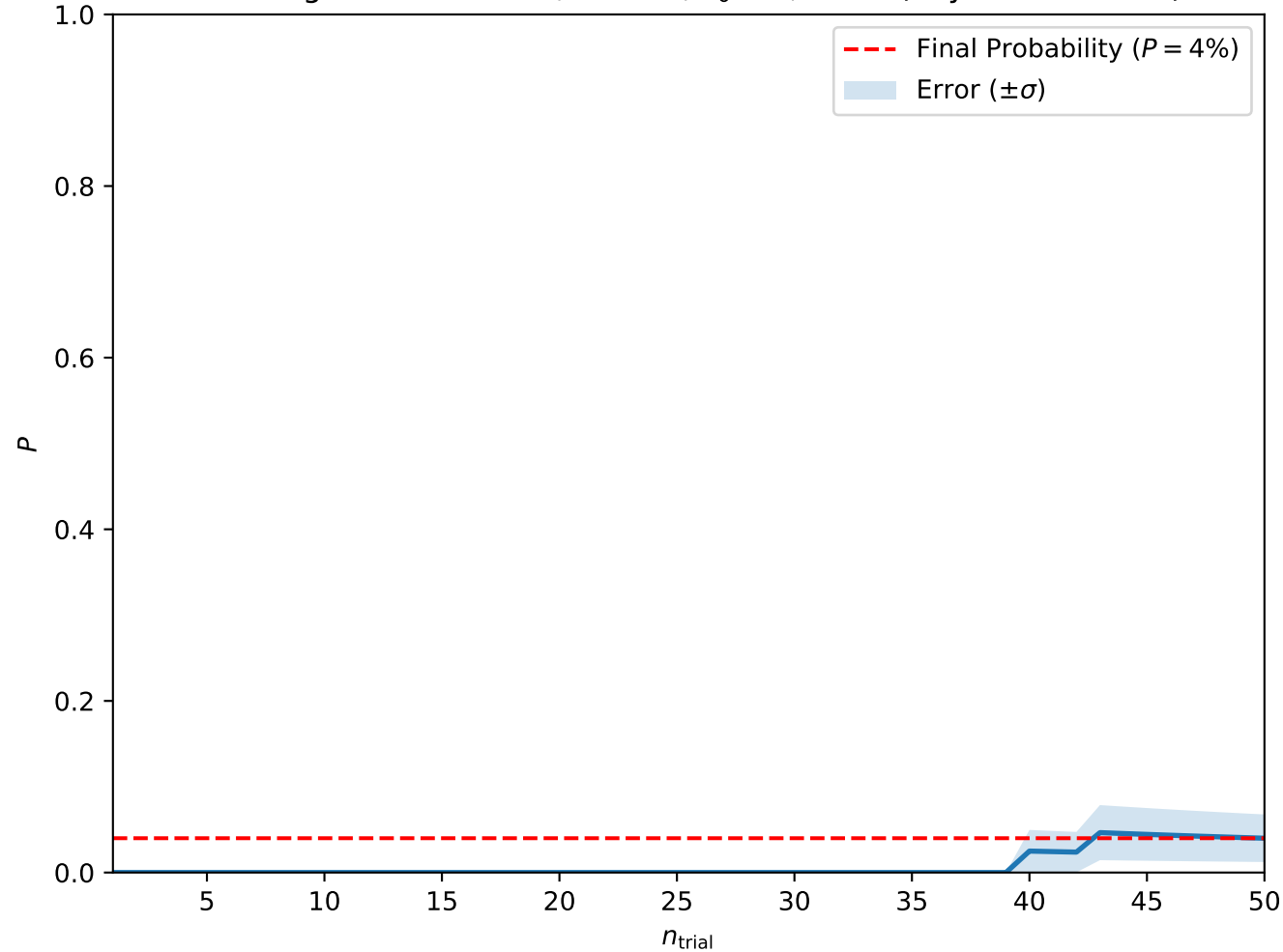
Convergence at A = 0.3, H = 0.3, T_0 = 1, w = 5 (Skyrmion Lattice)
