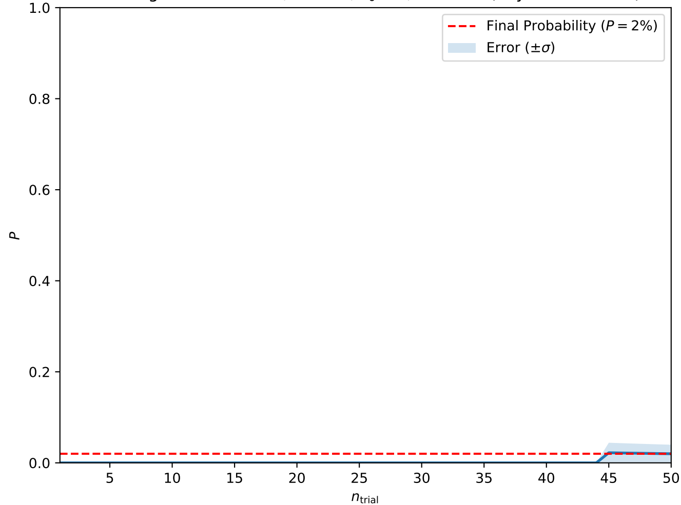
Convergence at A = 0.3, H = 0.3, T_0 = 3, w = 1.25 (Skyrmion Lattice)
