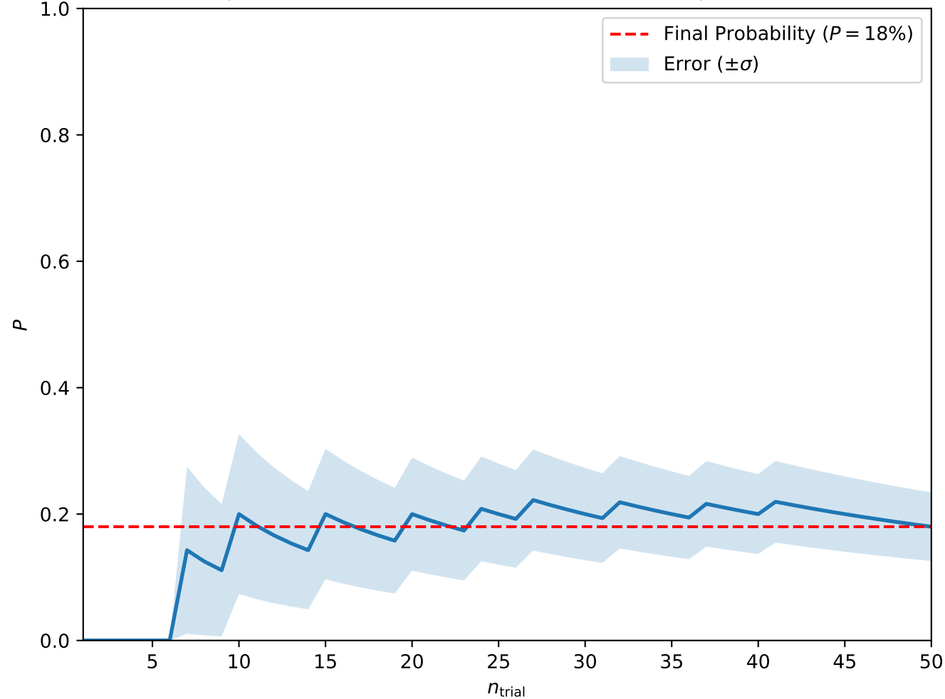
Convergence at A = 0.3, H = 0.3, T_0 = 3, w = 5 (Skyrmion Lattice)
