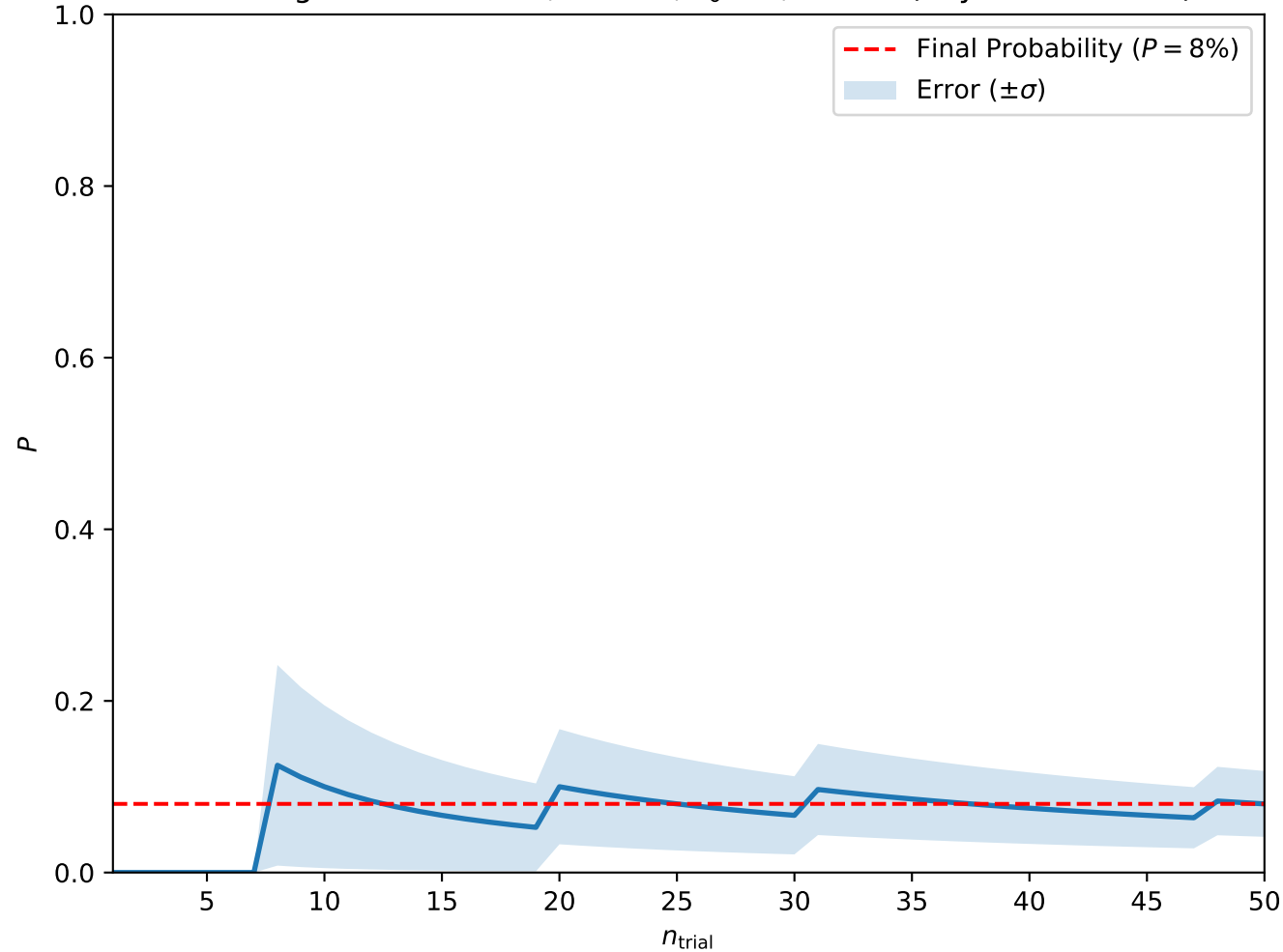
Convergence at A = 0.3, H = 0.3, T_0 = 5, w = 10 (Skyrmion Lattice)
