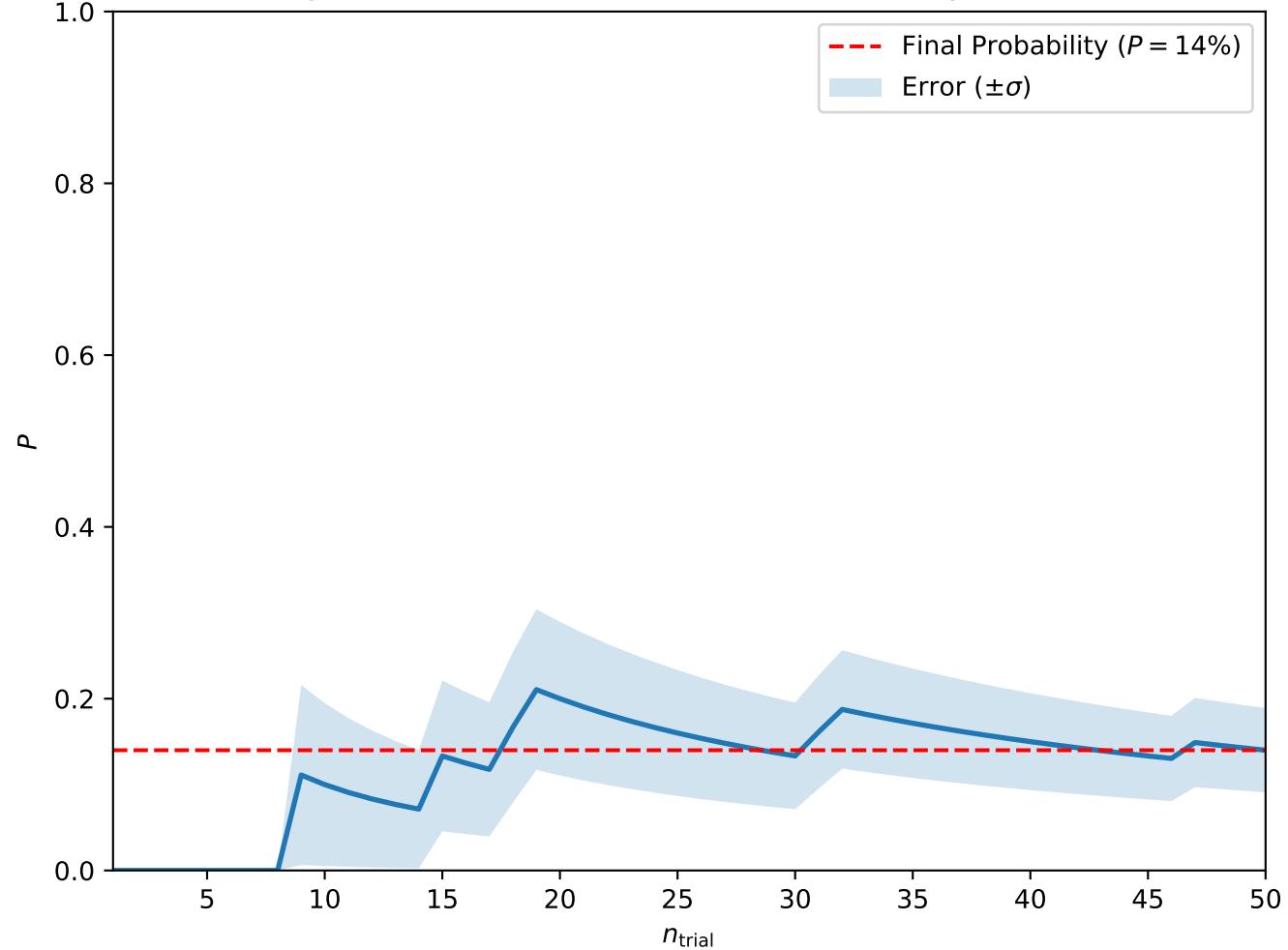
Convergence at A = 0.3, H = 0.3, T_0 = 5, w = 5 (Skyrmion Lattice)
