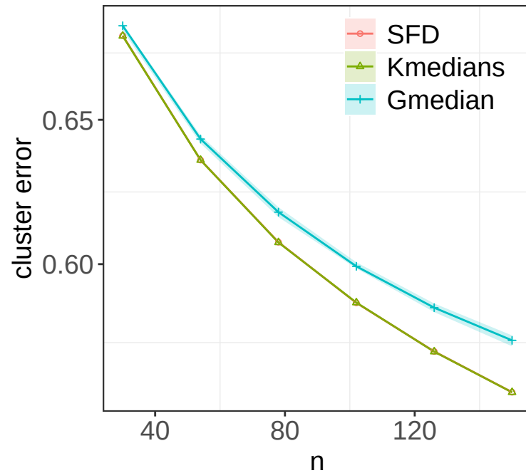
p = 10
