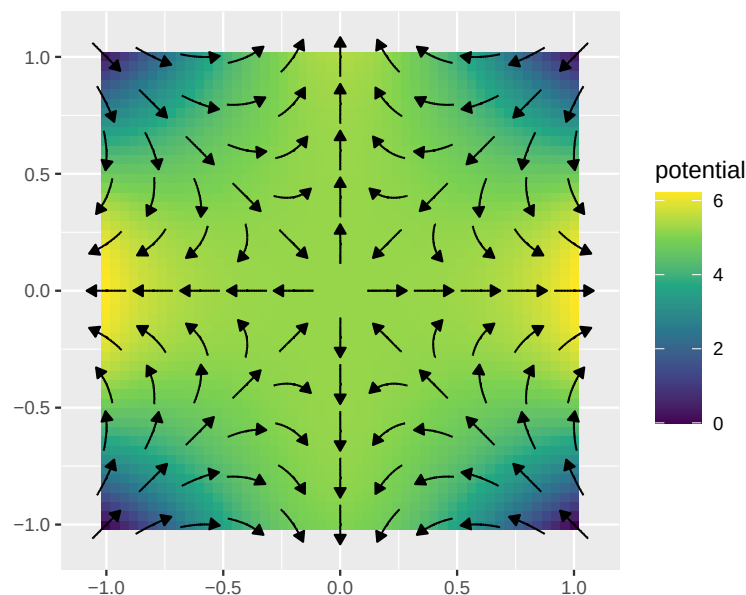
Figure 19: geom_potential() is the opposite of geom_gradient_field() : where the latter accepts a scalar field and plots a vector field, the former accepts a vector (gradient) field and plots the corresponding potential (scalar field).
