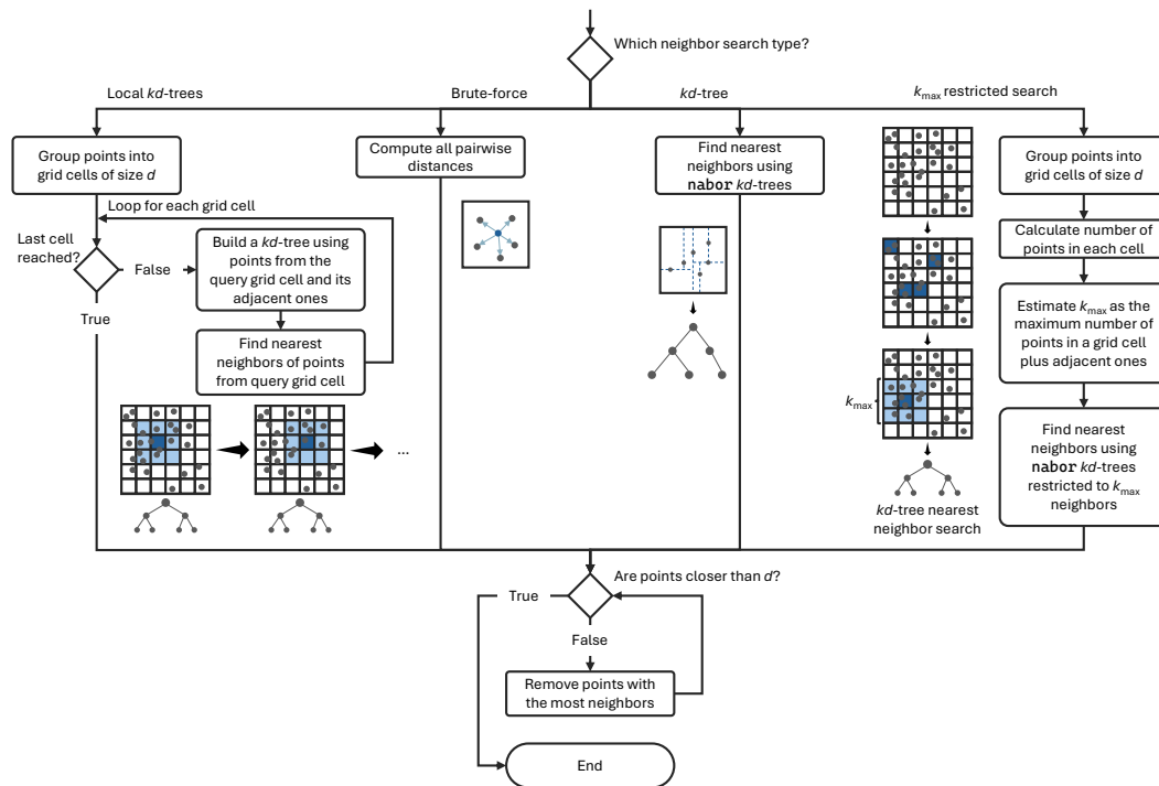
Figure 3: Diagram illustrating the four nearest neighbor search strategies implemented in GeoThinner for distance-based thinning. The methods include brute-force, standard kd-trees, local kd-trees, and restricted kd-trees using estimated k-max. Each approach computes neighboring points within a thinning distance before proceeding with point removal.
