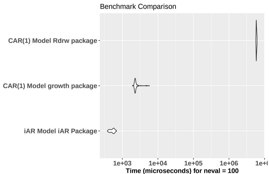
Figure 8: Distribution of the computation times (in microseconds) of the functions carma (growth package), drw (Rdrw package) and the loglik method (iAR package).
