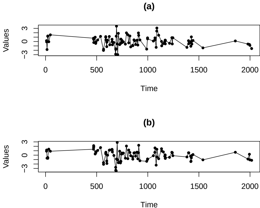
Figure 7: Simulated Bivariate Irregularly Observed Autoregressive process.
