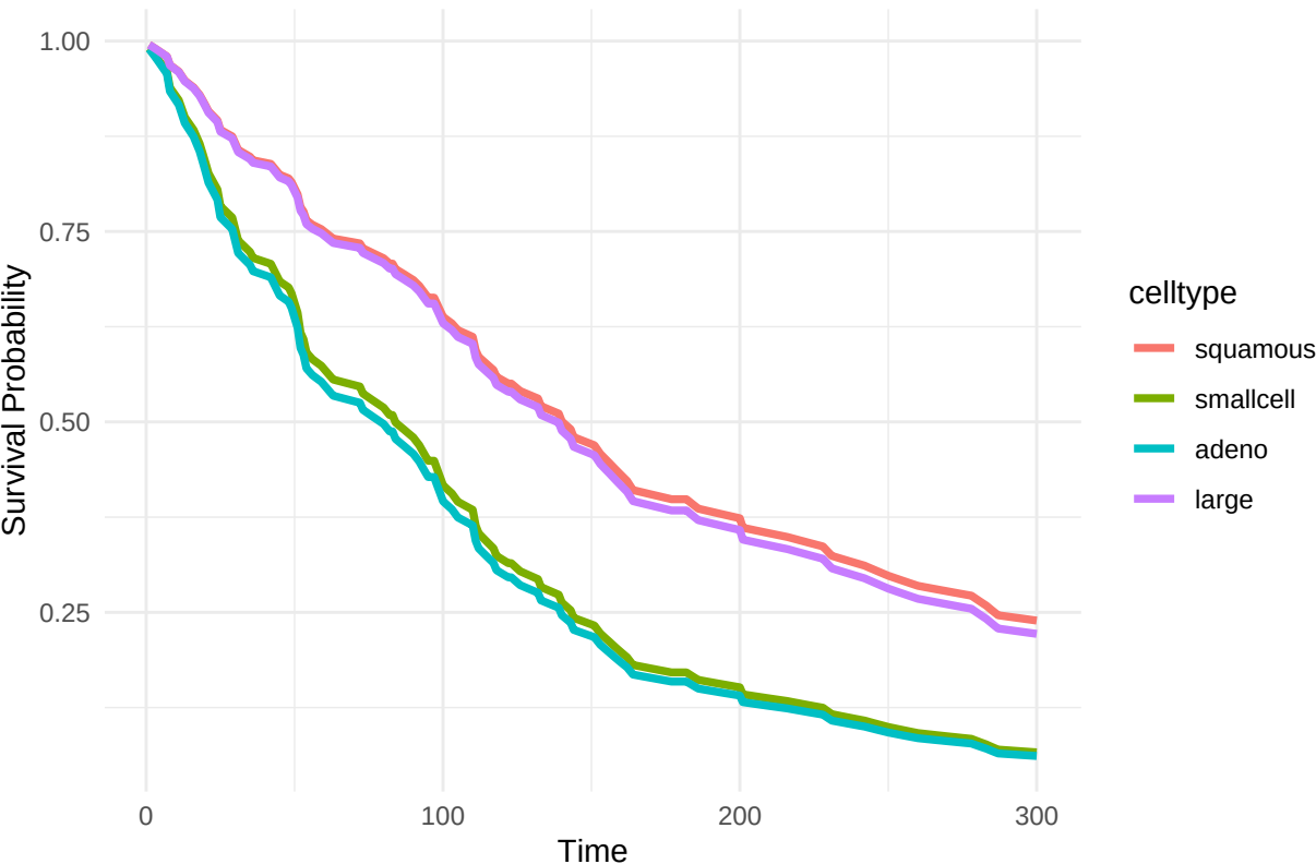
Mean Survival Curves by Celltype
