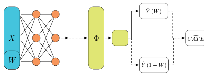
Figure 1: Estimating CATE Using Deep Neural Networks
