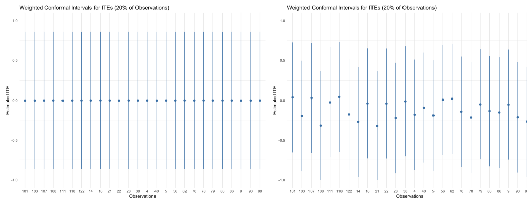
Figure 3: Conformal Predictions from Deep Neural Network-Based Meta Learners
