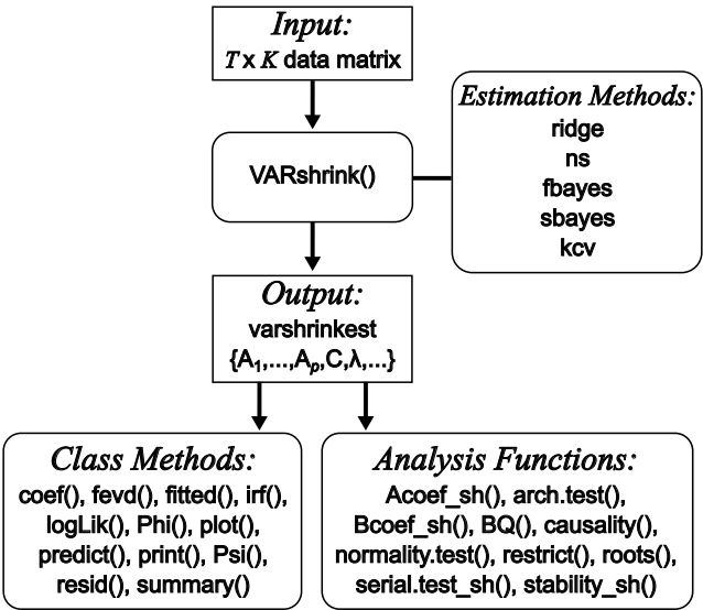
Figure 1: Systematic diagram of the VARshrink package.
