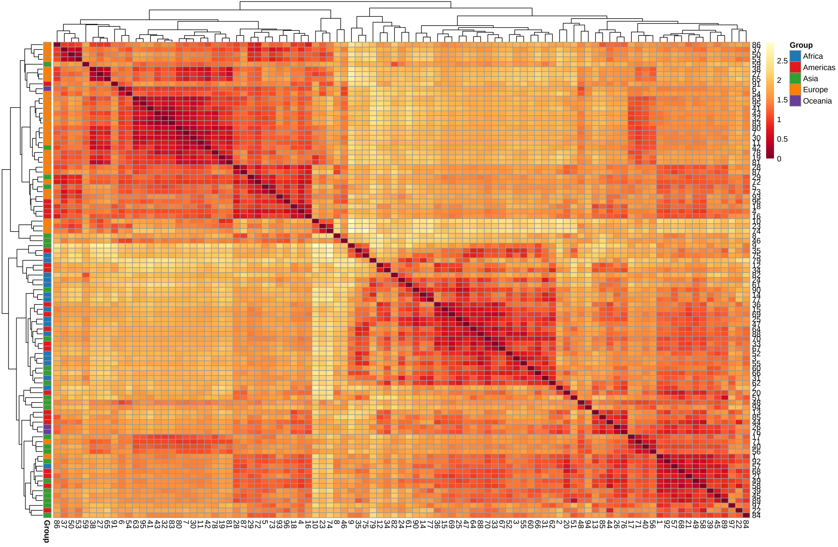
Heatmap for World Development Data with robust G-Gower (Continent)
