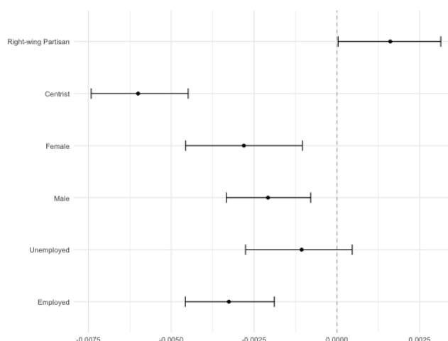
Figure 7: HTEs for Selected Covariates of Interest
