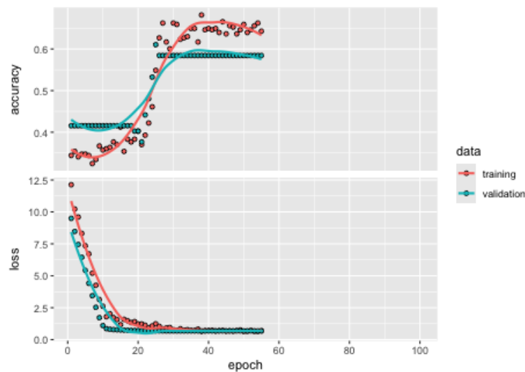
Figure 2: Accuracy Plot and Trace Plot of the Loss Function for the S-Learner
