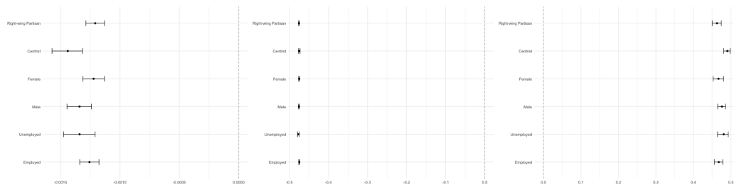
Figure 4: HTEs from Deep Neural Network-Based Meta Learners
