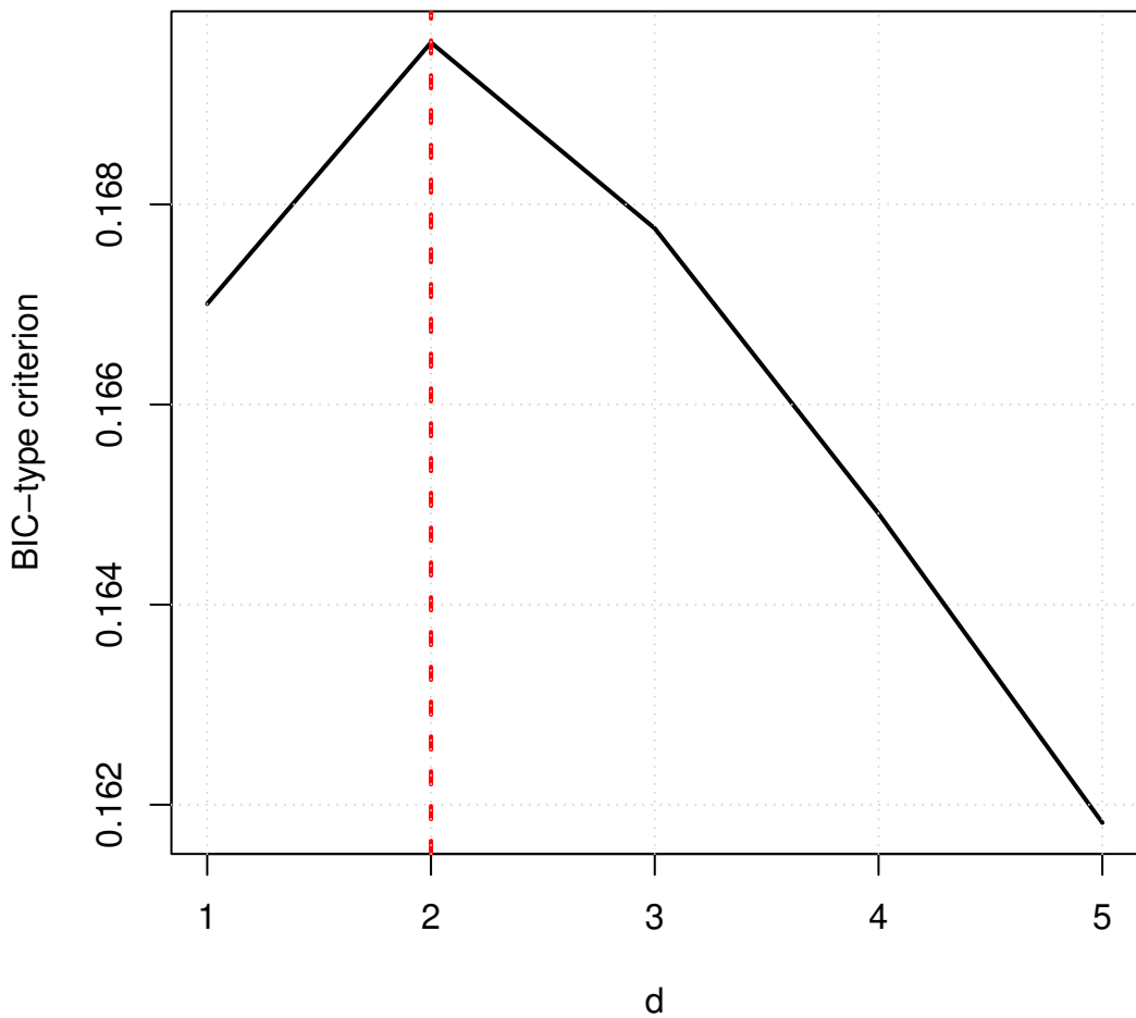
BIC-type curve at optimal \rho from CV
