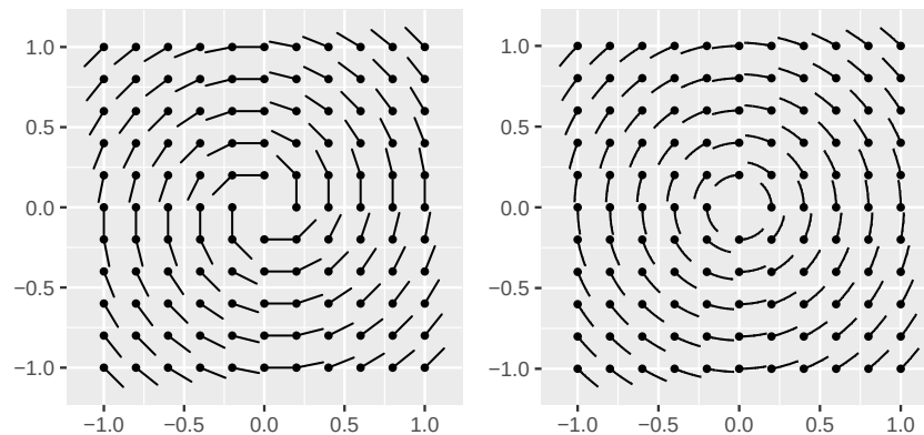
Figure 16: A stream version of geom_vector_field2() (left) is available as geom_stream_field2() (right).
