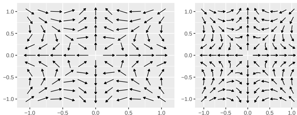
Figure 18: geom_gradient_field() can plot the gradient vector field of an input scalar function, computing it using numDeriv . Setting the type argument toggles between arrows and streams.
