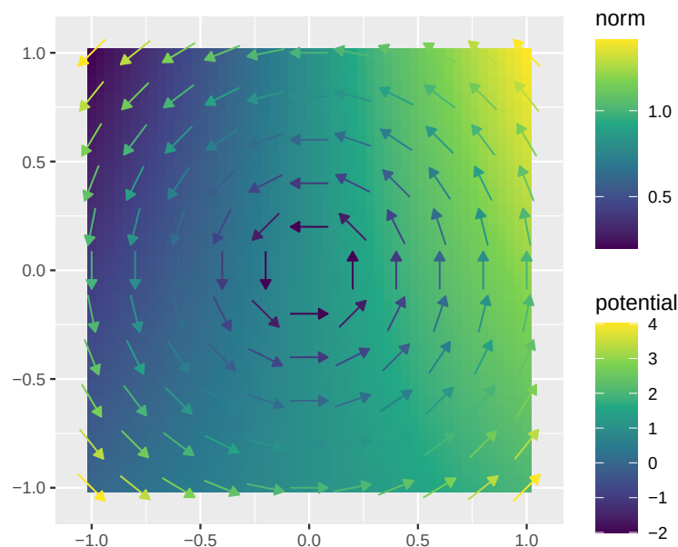
Figure 20: geom_potential checks if \mathbf{f}(x, y) is conservative by evaluating \partial f_y / \partial x - \partial f_x / \partial y . A warning is issued if significant deviations occur.
