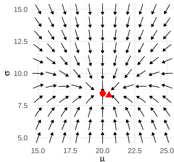
Figure 22: Gradient field of the log-likelihood function for normally distributed data of size n = 200 . The true value of the unknown parameter is illustrated with the red triangle; the MLE with the red circle. The learning rate corresponds to what was previously labeled average speed.
