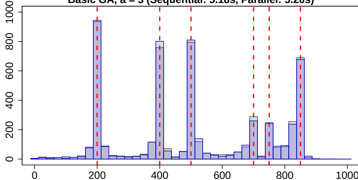
Basic GA, a = 3 (Sequential: 5.18s, Parallel: 5.20s)
