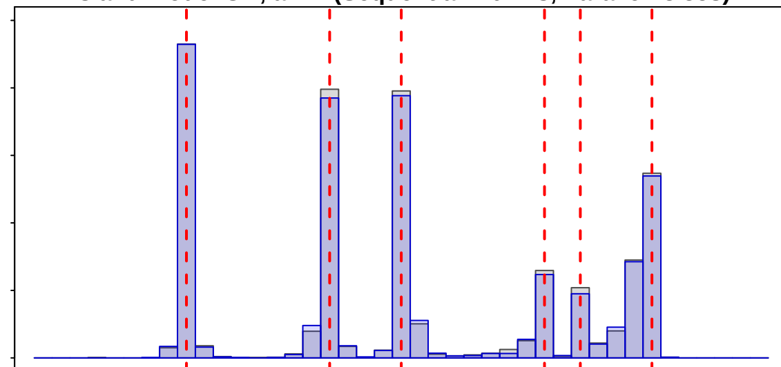
Island Model GA, a = 2 (Sequential: 10.21s, Parallel: 8.35s)
