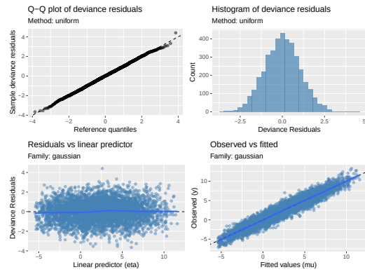
Figure 3: Example output from the diagnose function for a Gaussian model
