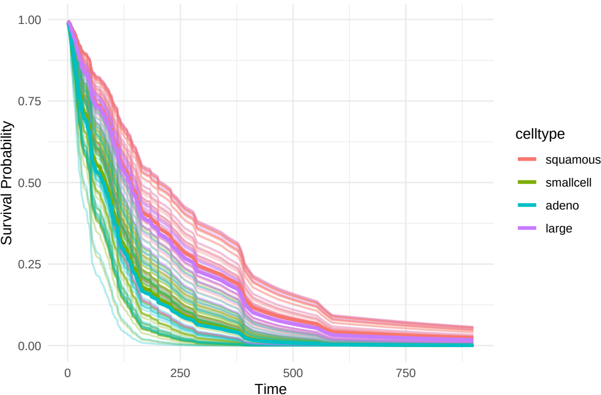
Survival Curves by Celltype
