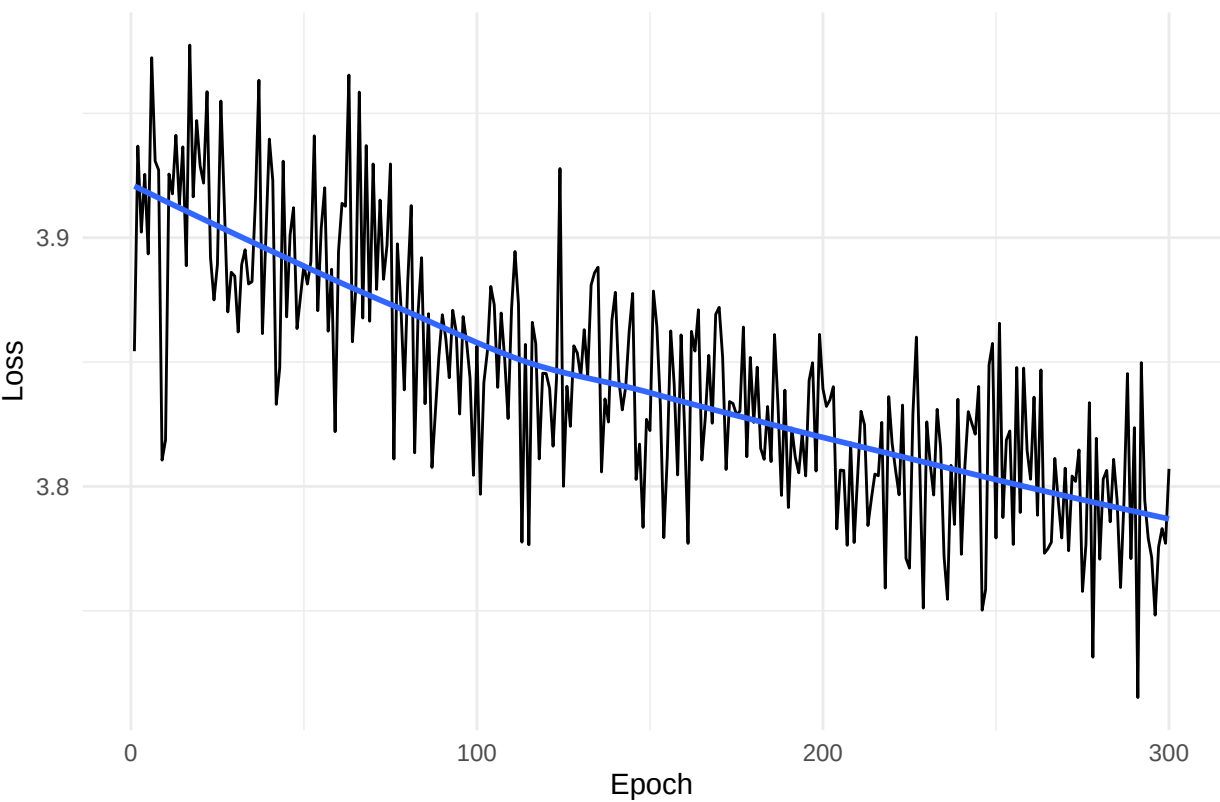
survdnn training loss
