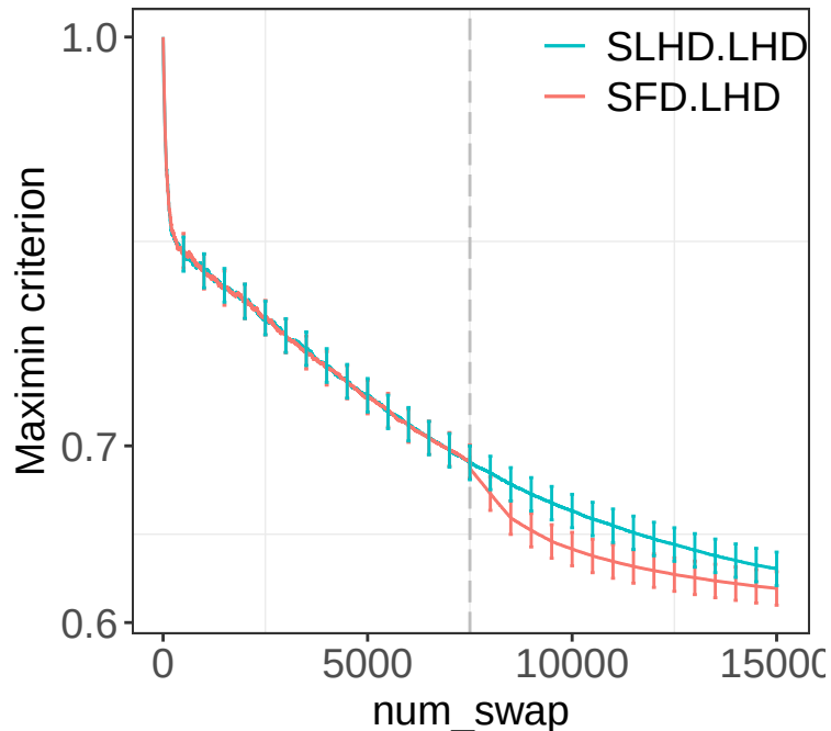
Maximin Design: p = 10 , n=100
