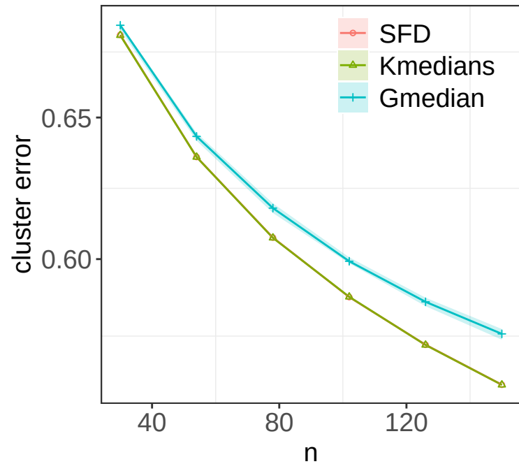
p = 10
