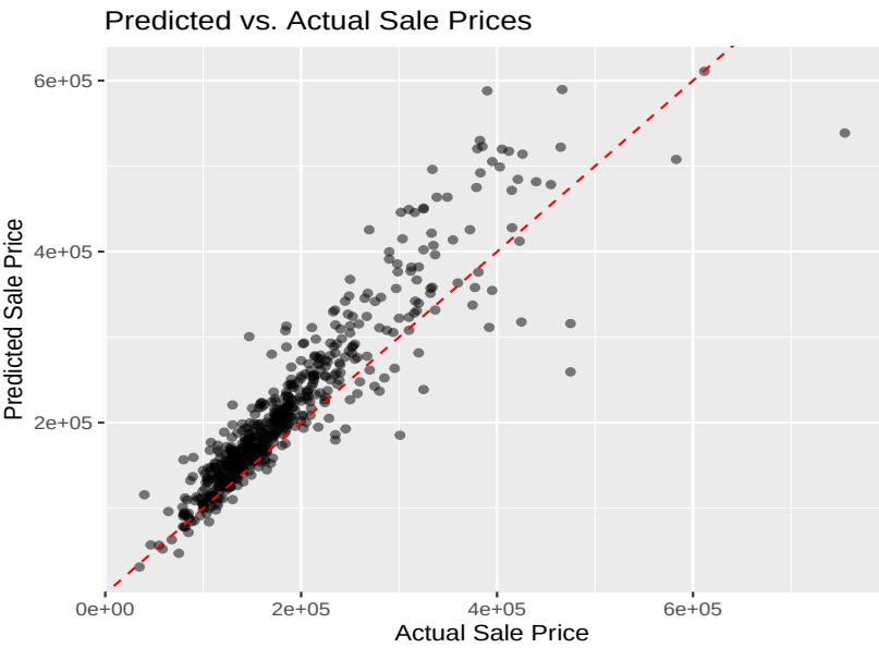
Figure 5: Predicted vs. Actual Sale Prices on the Test Set
