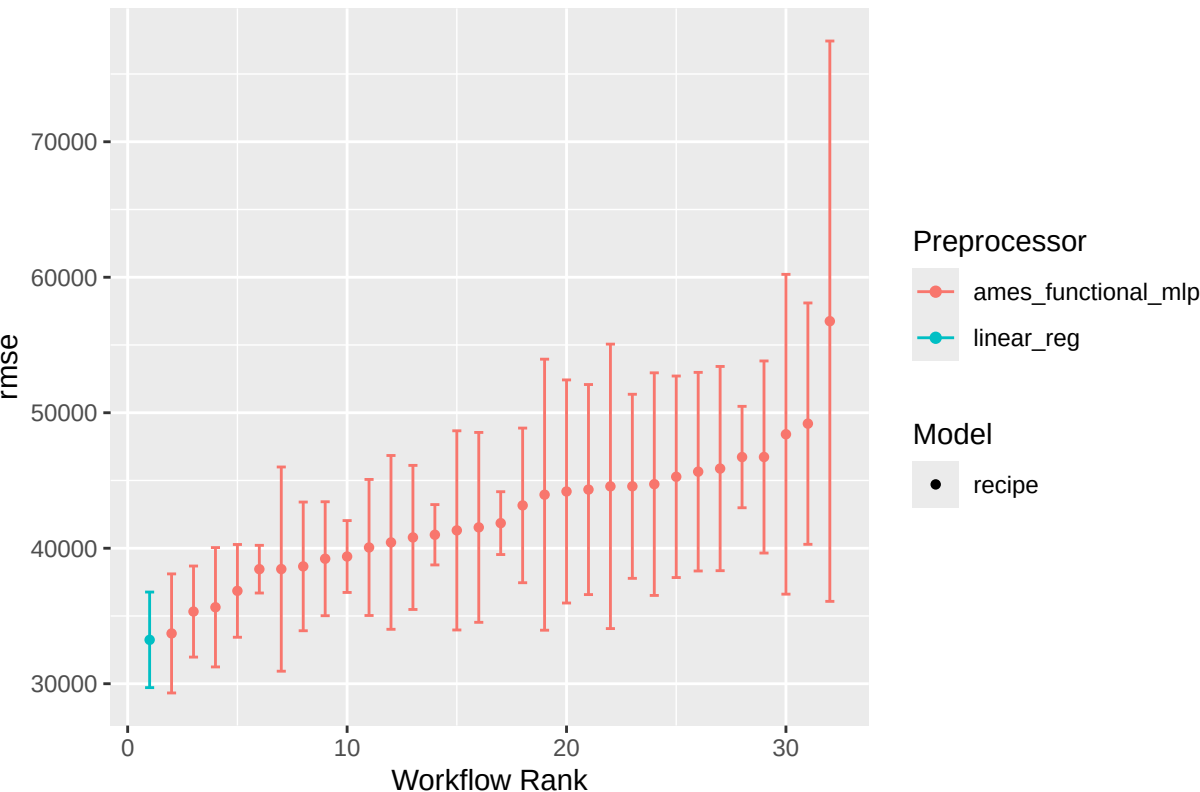
Comparison of Models using Workflowsets
