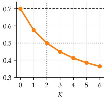
BT-implied preference probability
