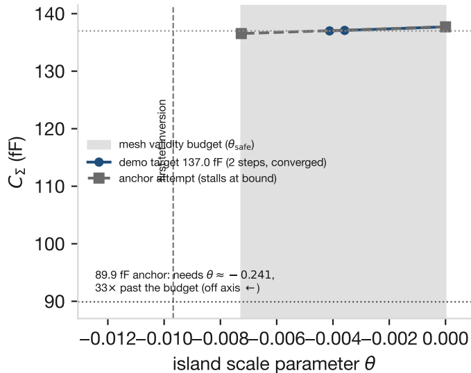
(b) Real 133k-tet device mesh: convergence within budget; anchor honestly out of reach
