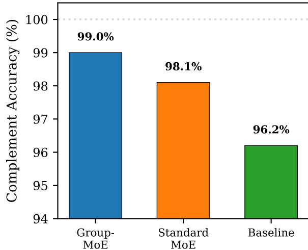
Composition Split (4→2)
