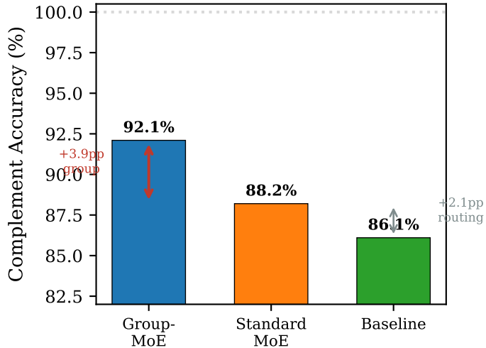
Complement Split (1→5)
