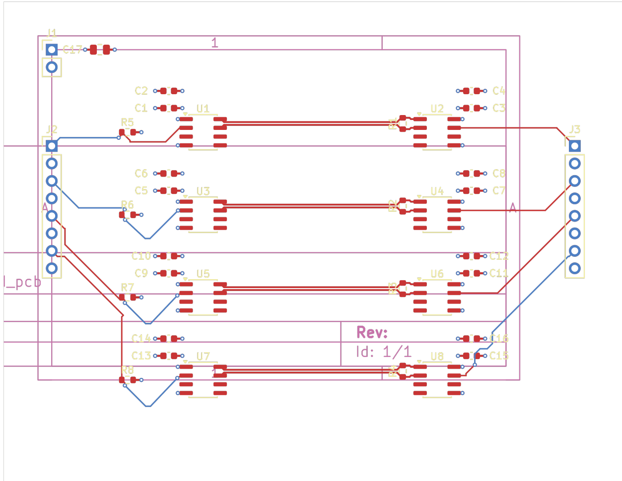
Figure 5: Assembly
