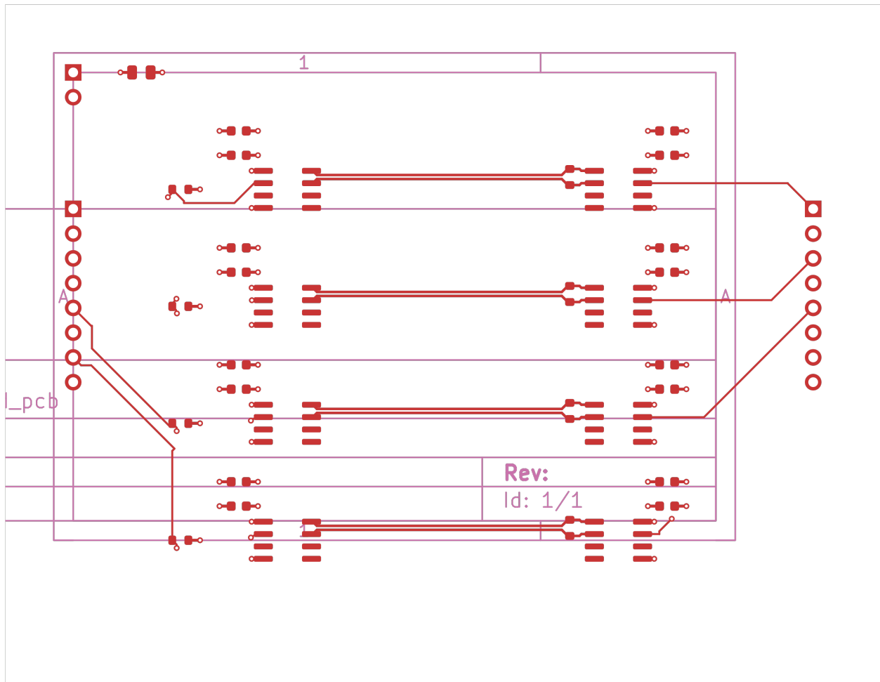
Figure 6: F.Cu
