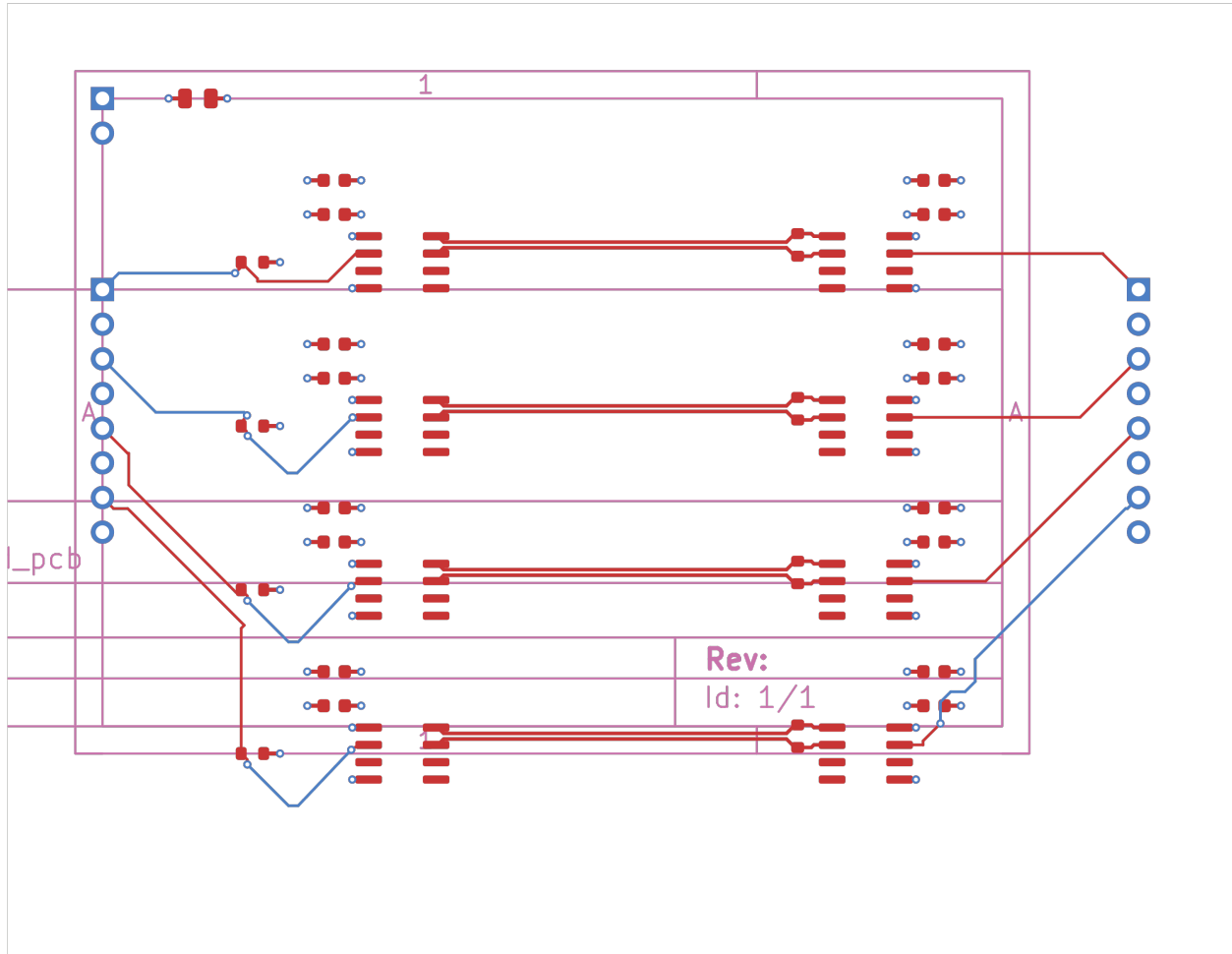
Figure 4: PCB Copper
