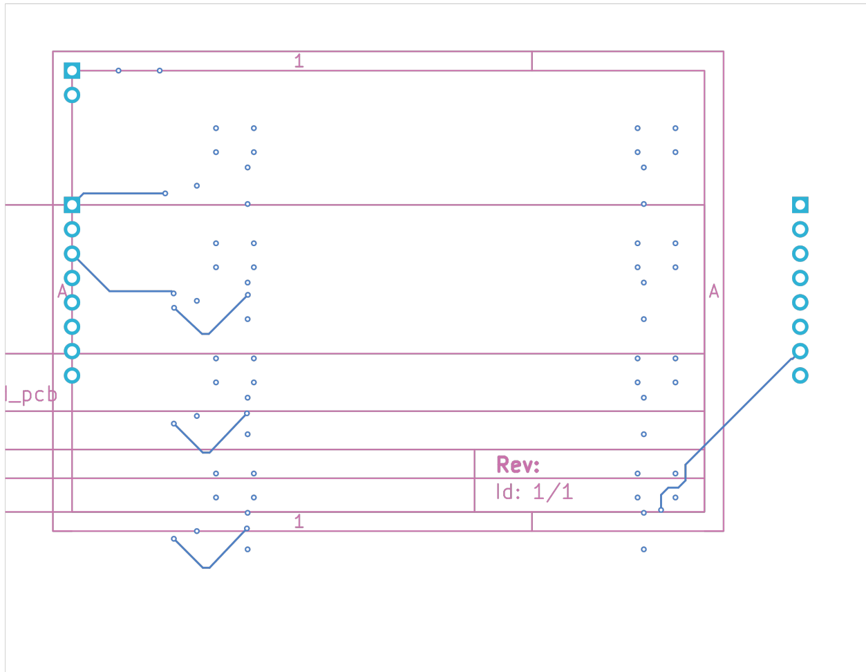
Figure 3: PCB Back
