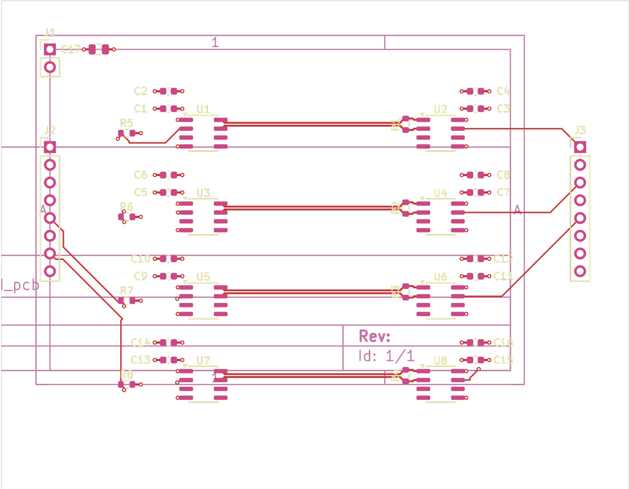
Figure 2: PCB Front
