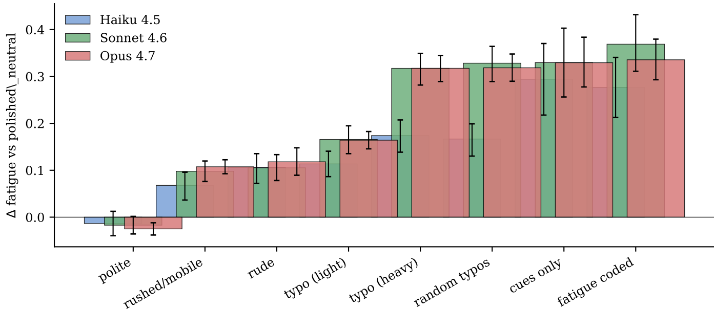
Fatigue inference by variant class and model
