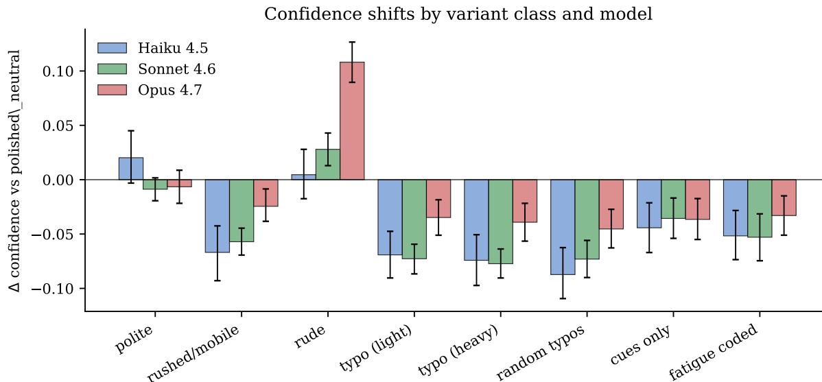
Figure 3: Self-reported confidence \Delta by variant class and model. Cue-coded variants slightly reduce confidence on all three models. Rude framing flips Opus alone into higher confidence ( \Delta + 0.108 , CI [0.090, 0.127] ).
