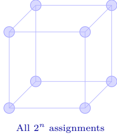
Figure 1: World-model architecture. (a) The free model admits all 2^n truth-value assignments as worlds. (b) The weather model excludes assignments violating \text{rain} \Rightarrow \text{clouds} (crossed vertices). (c) An abstract constrained model selects an arbitrary subset of the Boolean cube. Compositionality holds in all three; independence holds only in (a).
