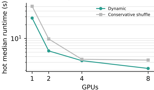
TPC-H Q9 SF1000 on B200 GPUs
