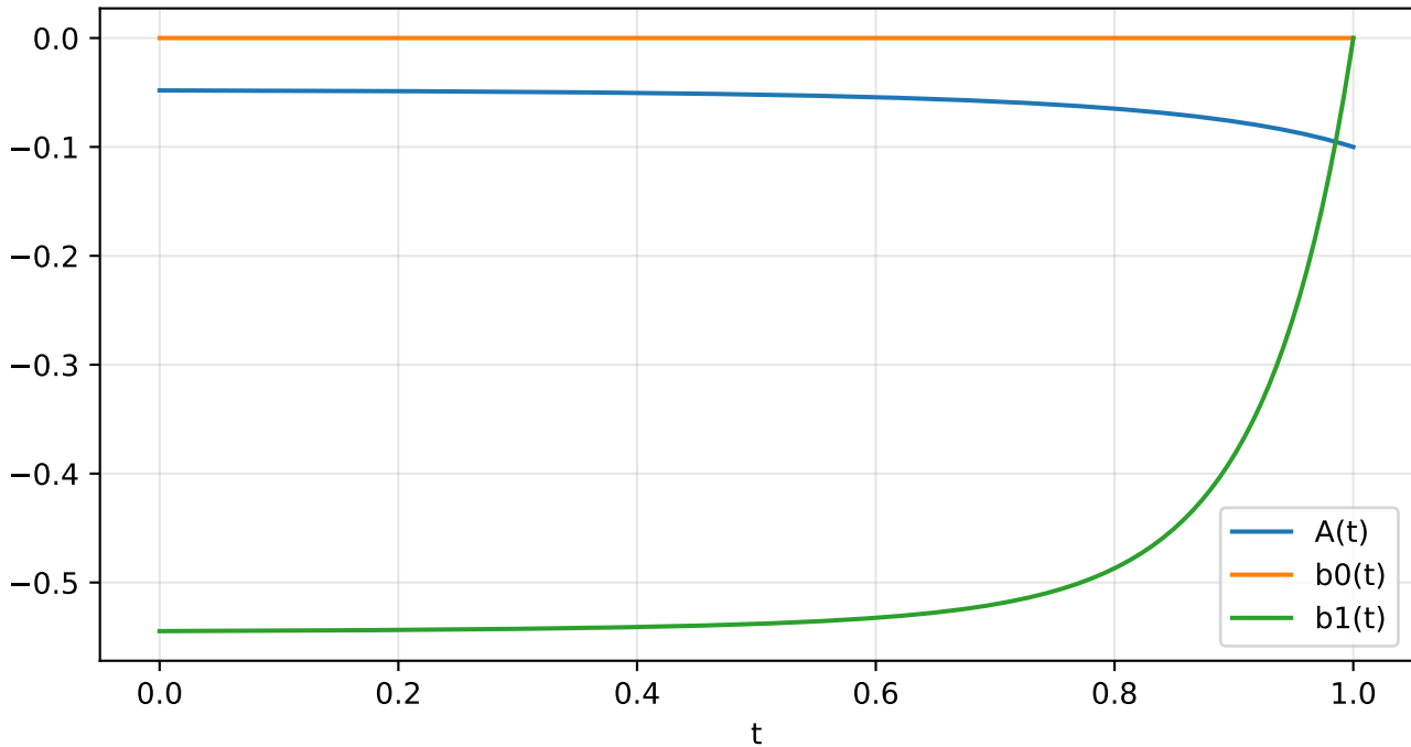
Coefficient Functions
