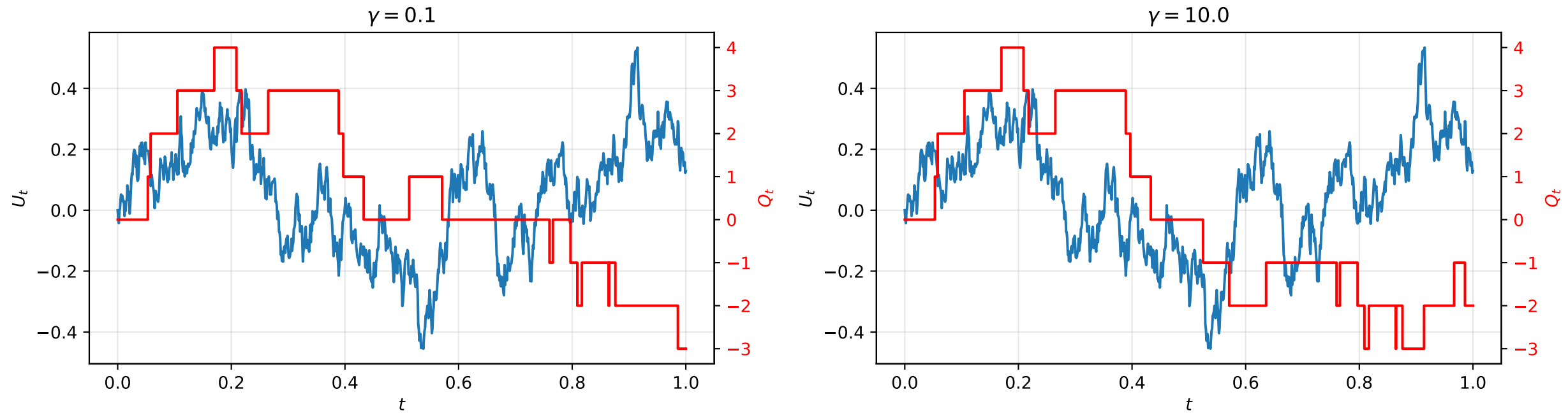
Figure 2. Fad and Inventory Paths under Different Gamma
