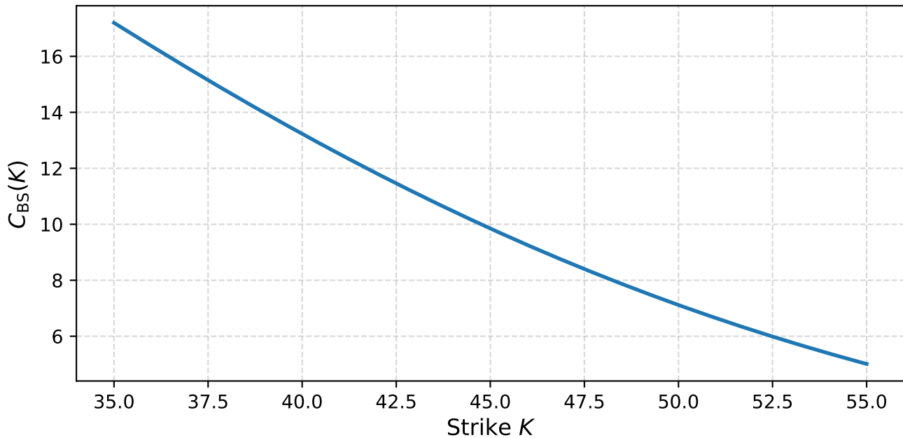
Black-Scholes call price as a function of K ( S_0 = 50 , r = 0.05 , \sigma = 0.30 , T = 1 )
