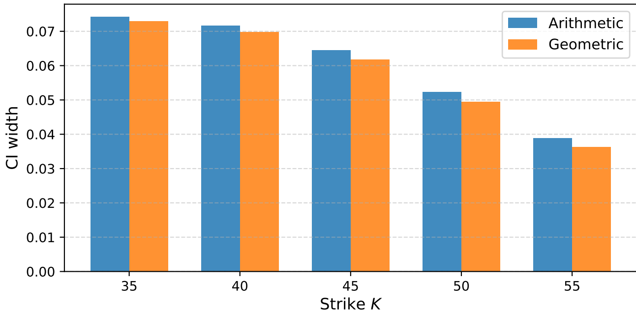
Width of 95\% confidence intervals: arithmetic vs geometric ( r = 0.05 , \sigma = 0.30 , T = 1 , M = 200,000 )
