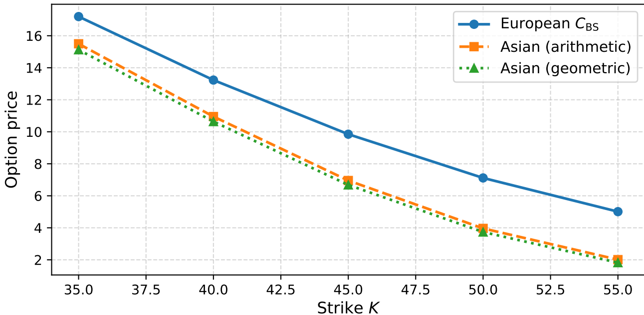
European vs Asian call prices ( r = 0.05 , \sigma = 0.30 , T = 1 , S_0 = 50 )
