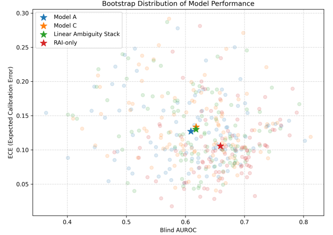
Figure 6. Bootstrap distribution of model performance across 1,000 resamples, comparing the blind AUROC against ECE.
