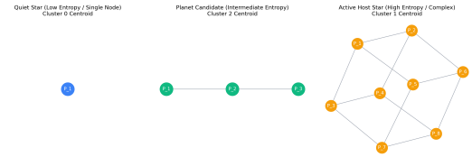
Figure 14. EXP-010: Representative alias graph topologies near each GMM cluster centroid: (Left) quiet star low-entropy single-node topology, (Middle) exoplanet intermediate-entropy path topology, (Right) active host star high-complexity high-entropy topology.
