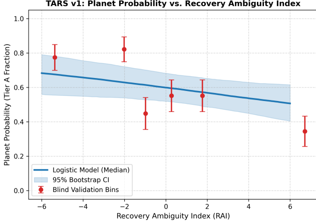
Figure 7. Calibrated logistic link model for the planet probability as a function of the standardized RAI, with 95% bootstrap confidence intervals.
