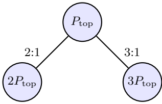
Figure 5. Representation of an exoplanet candidate alias graph. Vertices denote period hypotheses, and edges represent matched harmonics within phase tolerance \epsilon = 0.05 .
